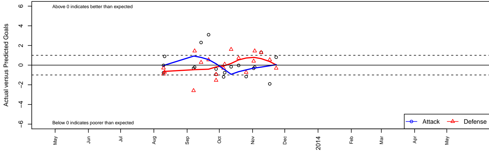
Beach FC G02 Dots are actual minus expected GF (blue circles) and GA (red triangles). Blue line is smoothed change in attack strength. Red is smoothed change in defense strength.
